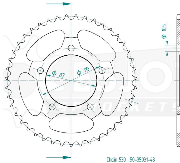
Chain 530 , 50-35031-43
