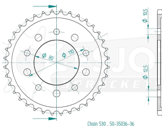
Chain 530_50-35036-36
