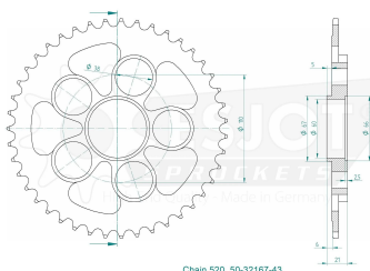
Chain 520, 50-32167-43
