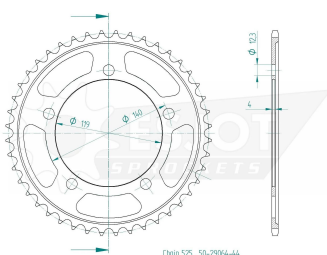
Chain 525 , 50-29064-44
